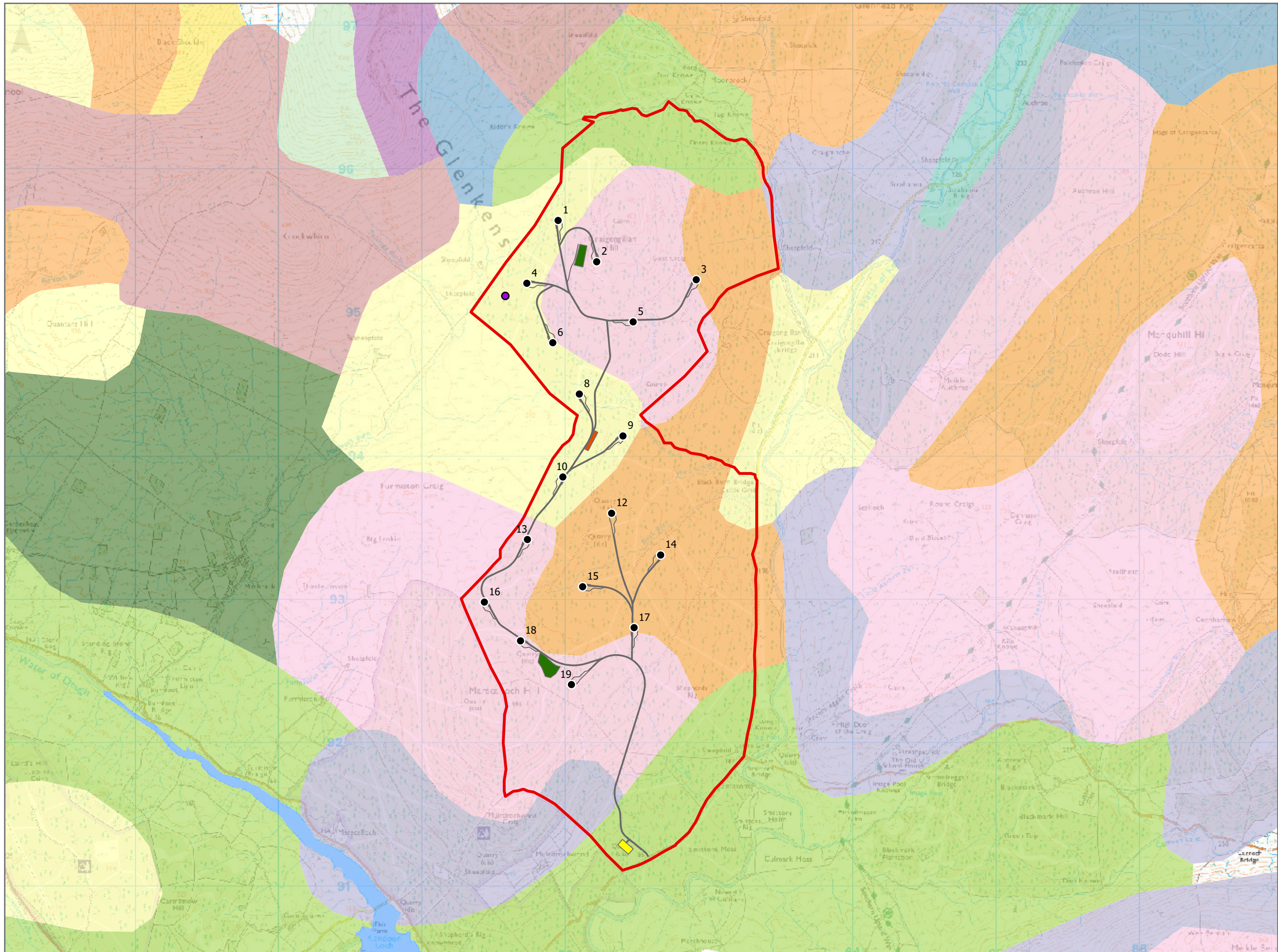
Figure 12.3: National Soils of Scotland
